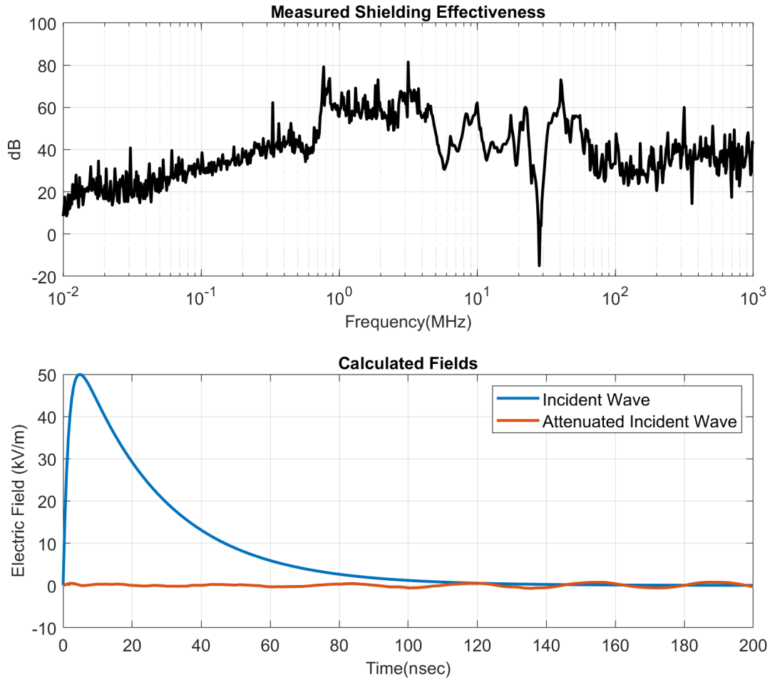
Figure 3-11 Measured shielding effectiveness and incident field calculation results for the substation control house constructed of six-side metal panels with welded seams (Type 4)
