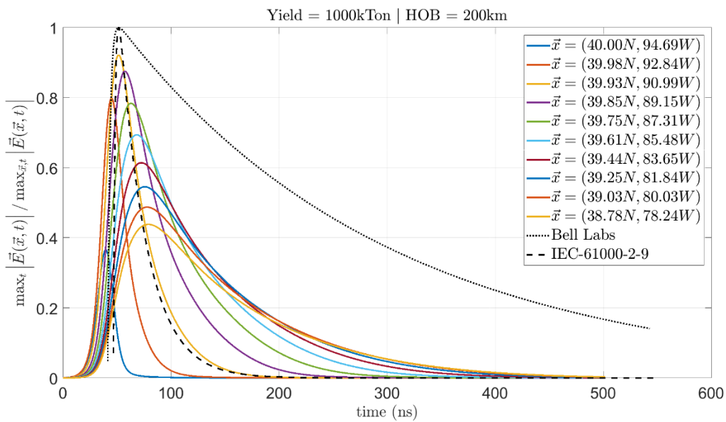
Figure 2-2 Normalized E1 EMP waveforms from benchmark 5 for ground locations generally east of ground zero (40° N, 95° W)
