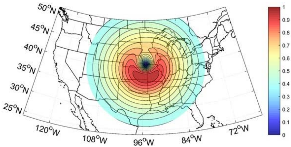
Figure 2-1 Normalized smile diagram for benchmark 5 (Yield = 1,000 kT, HOB = 200 km); ground zero location is 40° N, 95° W
